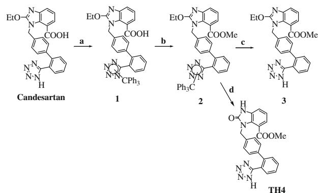
Scheme 1. Reagents and conditions: (a) TEA, trityl chloride, CH 2 Cl 2 ; (b) MeI, K 2 CO 3 , DMF, room temperature, 15 min; (c) HCl (1 N), DMF, 65–70 °C, 1 h; (d) HCl (1 N), DMF, 90 °C, 1.5 h. For [ 11 C]methyl-candesartan: (b) [ 11 C]MeI, K 2 CO 3 , Kryptofix, DMF, 65–70 °C, 3 min; (c) HCl (1 N), DMF, 65–70 °C, 2 min. For [ 11 C]TH4: d) HCl (1 N), DMF, 90 °C, 2 min.
