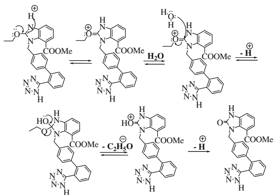
Scheme 2. Proposed mechanism for the conversion of the ethoxy group in methyl-candesartan to cyclic urea in TH4.
